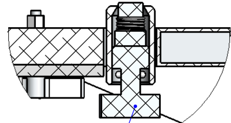
Friction brake B-B 1:2
